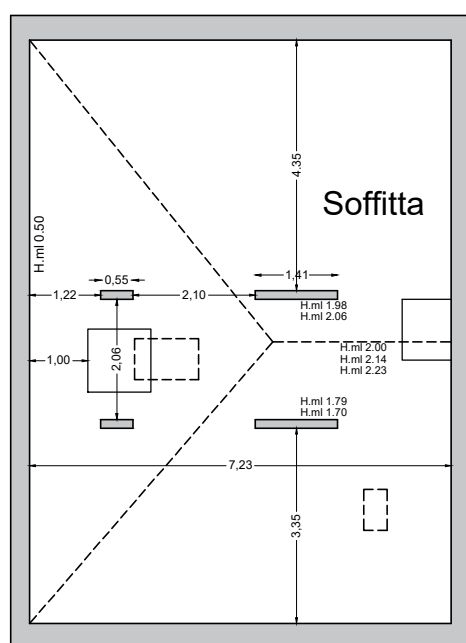
Piano Soffitta
