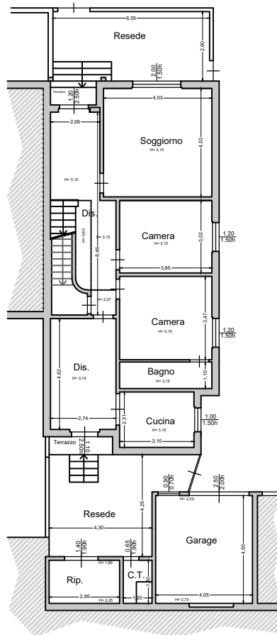
Piano Terra
