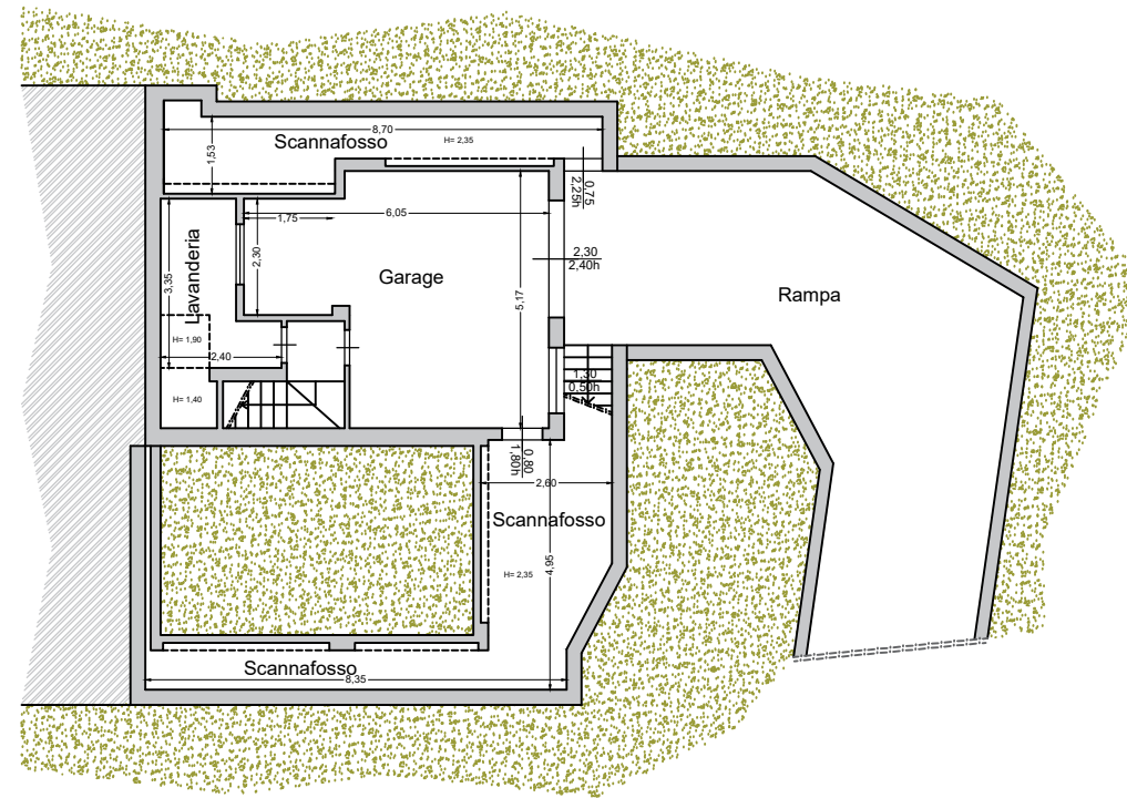
Piano seminterrato
