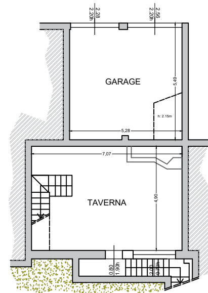
Pianta Piano Seminterrato h: 2.70m
